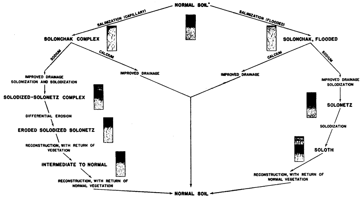
FIGURE 3.—An outline of the cycle of evolution of the intrazonal soils, Solonchak, Solonetz, and Soloth. It may be noted that these are not mutually exclusive categories but that many transitional soils are found, especially in those cases where the intrazonal soils occur with the normal soils as a complex.
