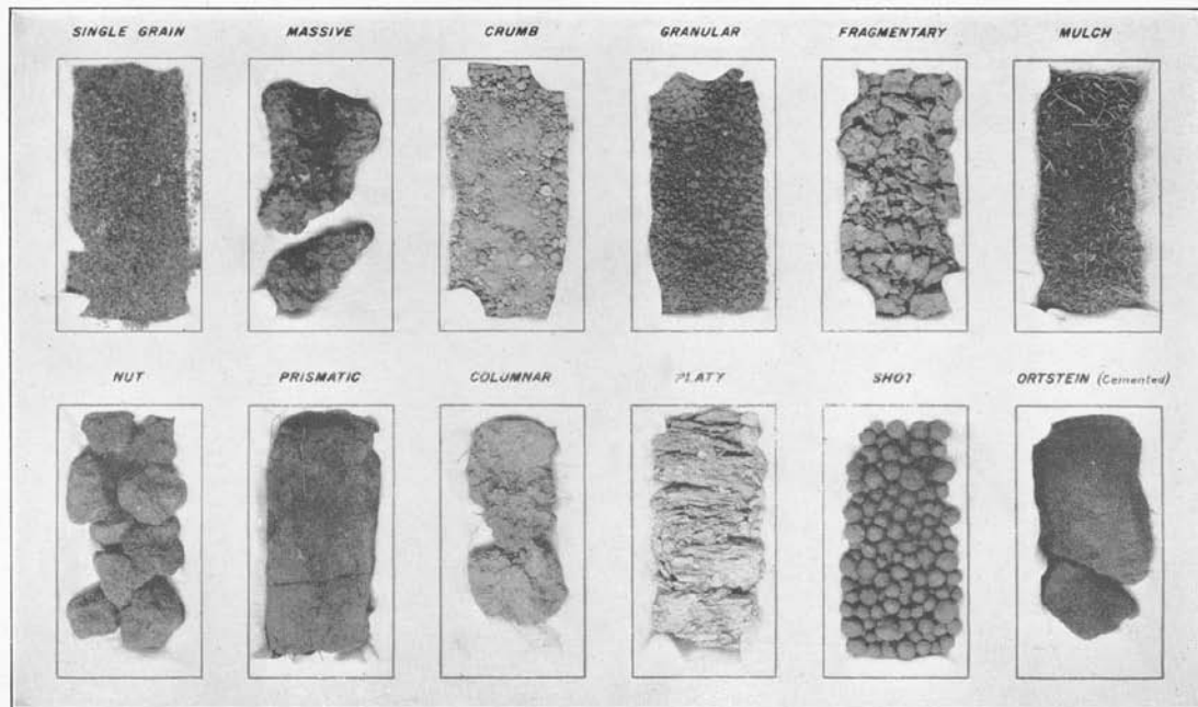
Several important types of soil structure. All of these structural types are produced through the operation of soil-building processes, except that the single grain, fragmentary, and massive may be developed or may be inherited from the parent material. The structure of soils is of great importance in studying their genesis or ecological relationships. (About one-fourth actual size.)
